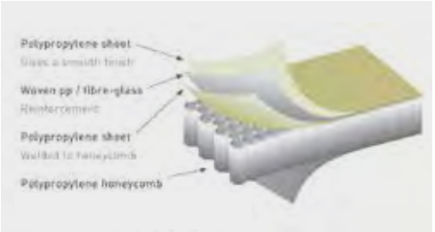
One piece Honeycomb Floor. Advanced one-piece seamless flooring solution that is up to 40% lighter than standard 12mm plywood yet much tougher,
